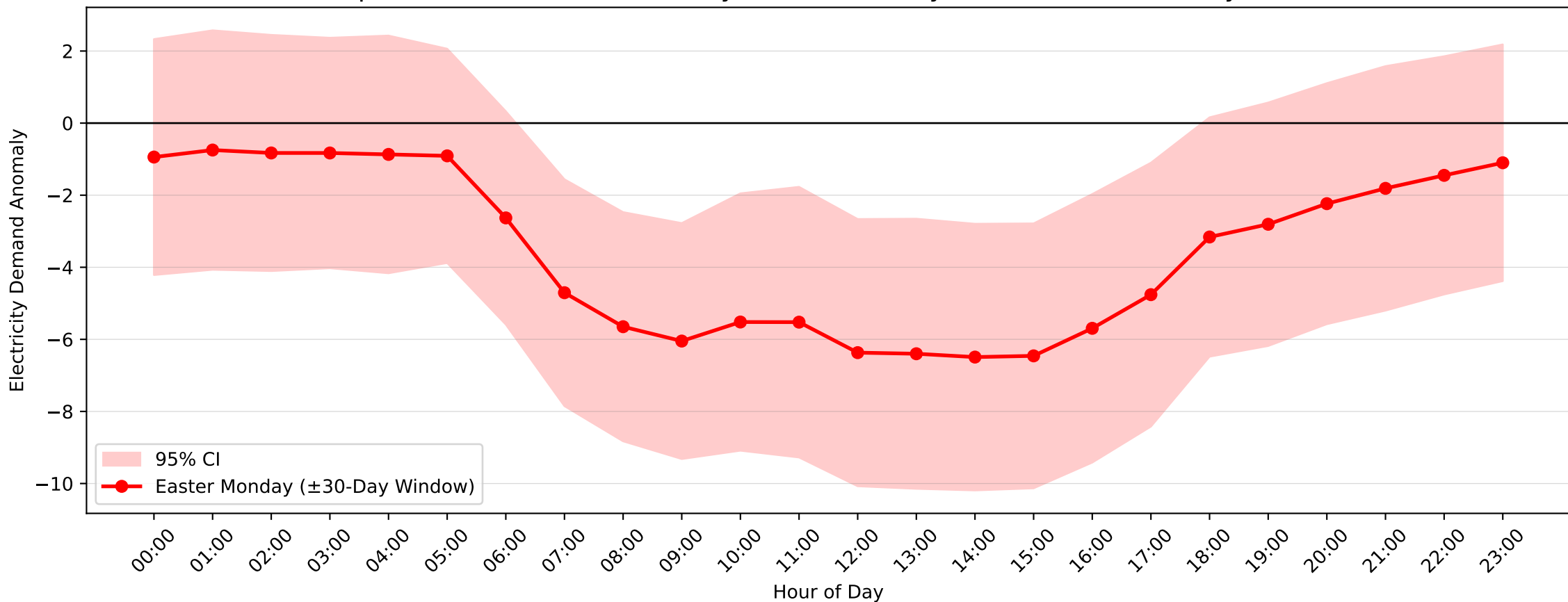
Macquarie Park Demand Anomaly: Easter Monday (2004-2017, \pm 30 -Day Window)
